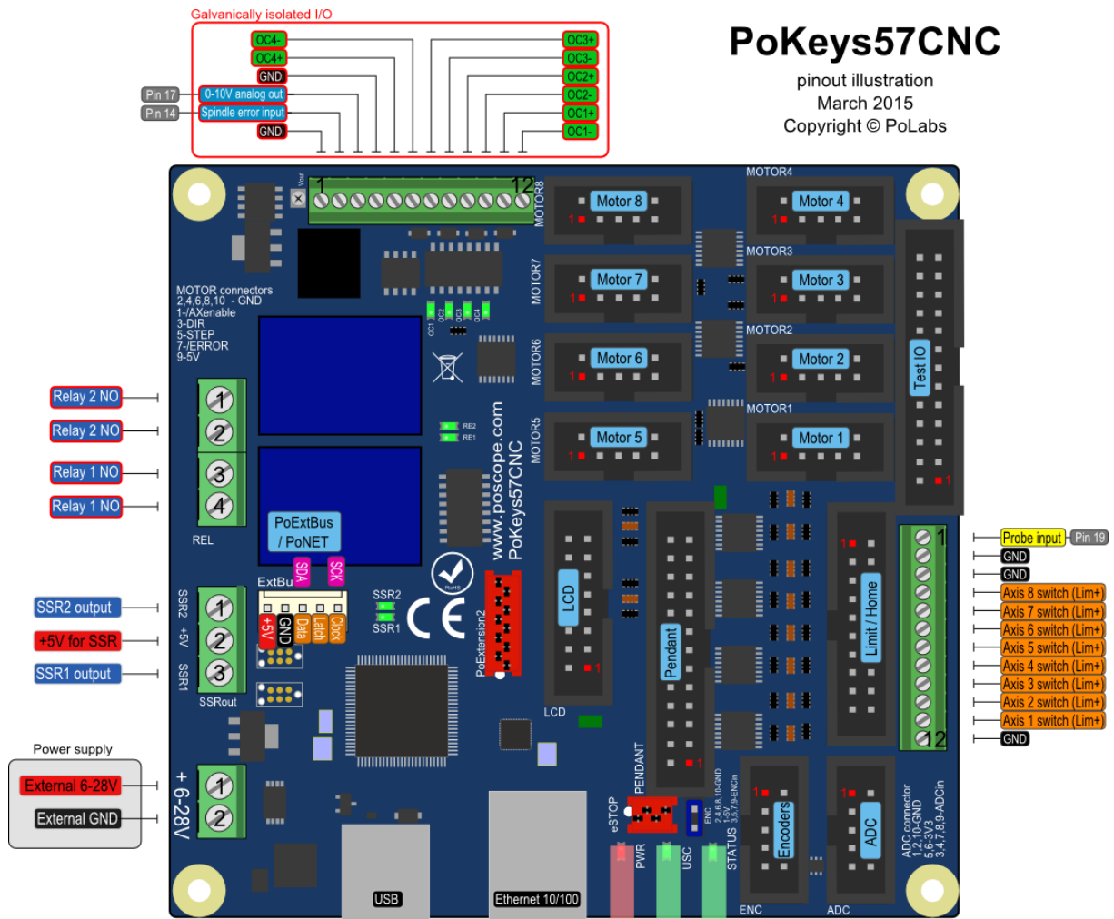
Motor connectors 1-8
