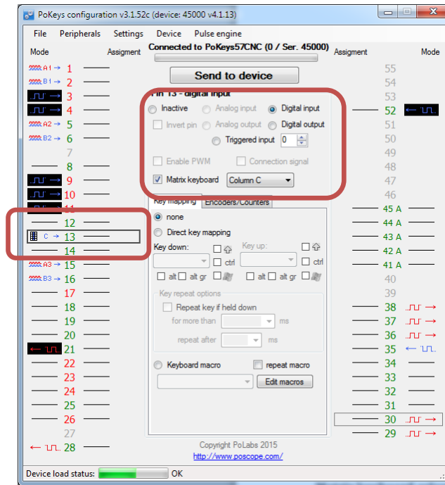
Figure 15: Assigning row and column pins
